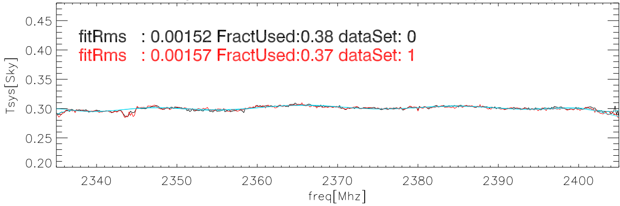
19nov12 Averaged data and fit for CalDeFlection/Tsys on Sky polB
