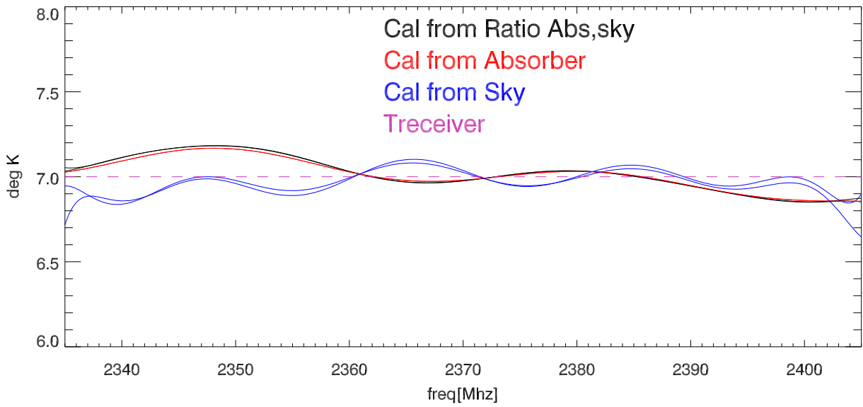
19nov12Cal in Kelvins vs freq polA
