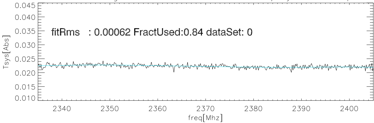
19nov12 Averaged data and fit for CalDeFlection/Tsys on Sky polA
