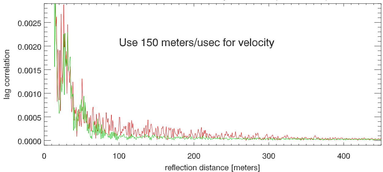
autoCorrelation vs round trip distance (150m/usec)
