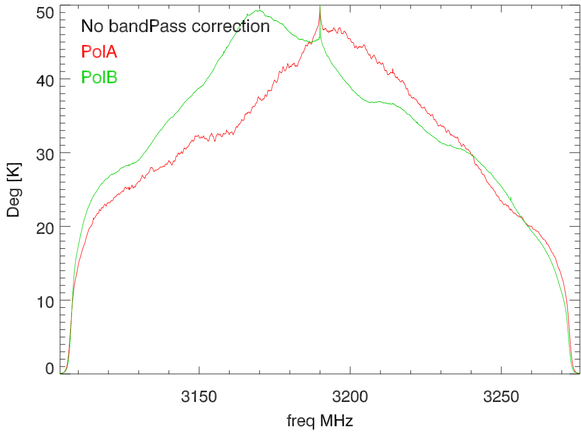
20jul20 sbh 110 min average spectra tracking blank sky. 3190MHz
