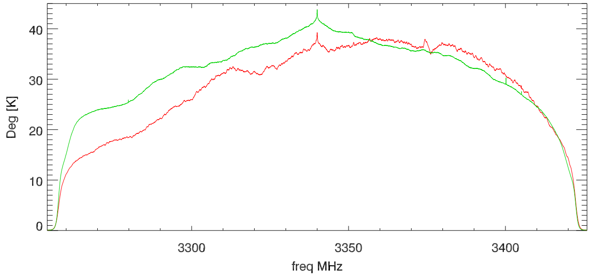
sbh 5min average spectra starting at 15:45
