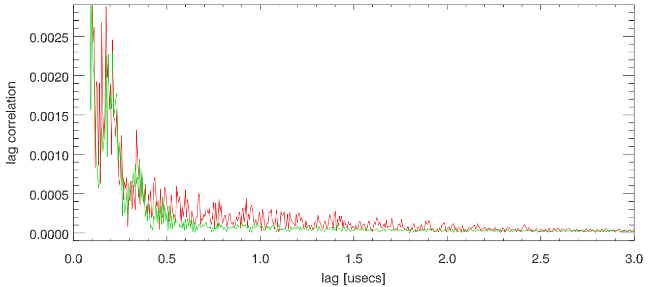
autoCorrelation (of 15:45 data) vs lag delay
