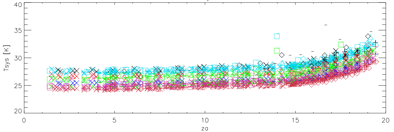
Sefd
