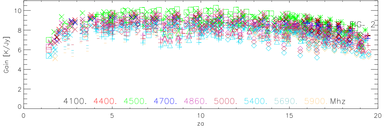
Tsys
