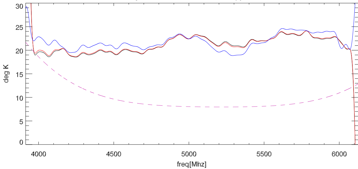
28jun12Cal in Kelvins vs freq polB
