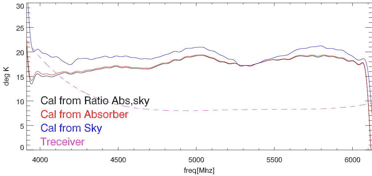
28jun12Cal in Kelvins vs freq polA
