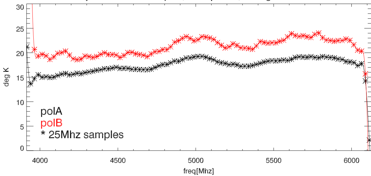
28jun12Cal in Kelvins polA,B overplotted, Average dataset fits
