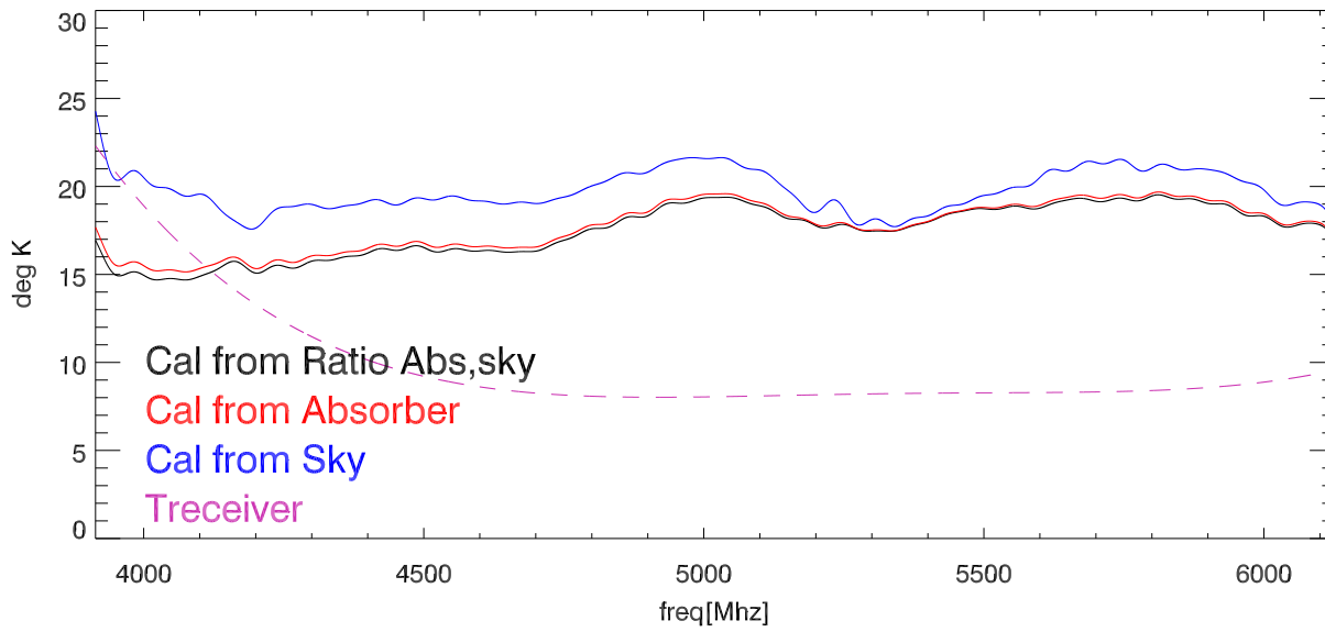
28jun12Cal in Kelvins vs freq polA
