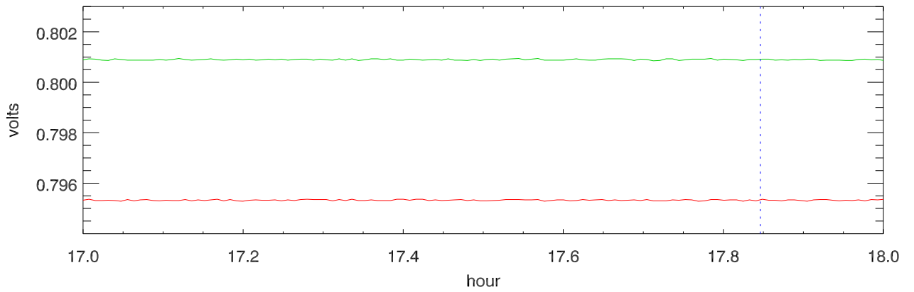
31may12 cband bias voltages stage: 1
