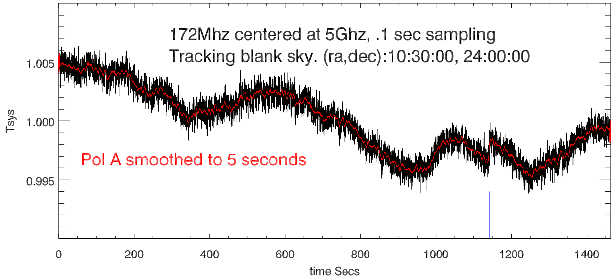
31may12 cband total power vs Time. PolA
