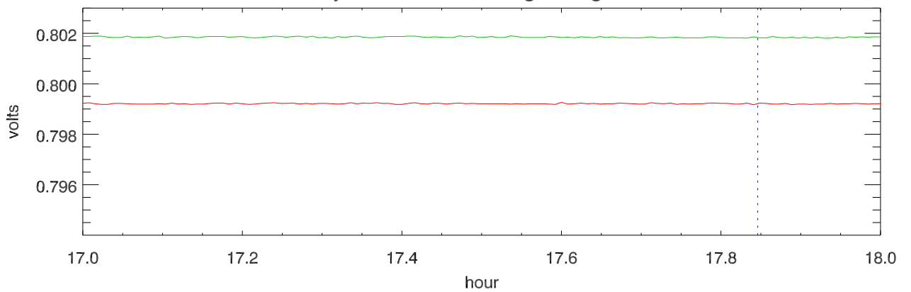
31may12 cband bias voltages stage: 2
