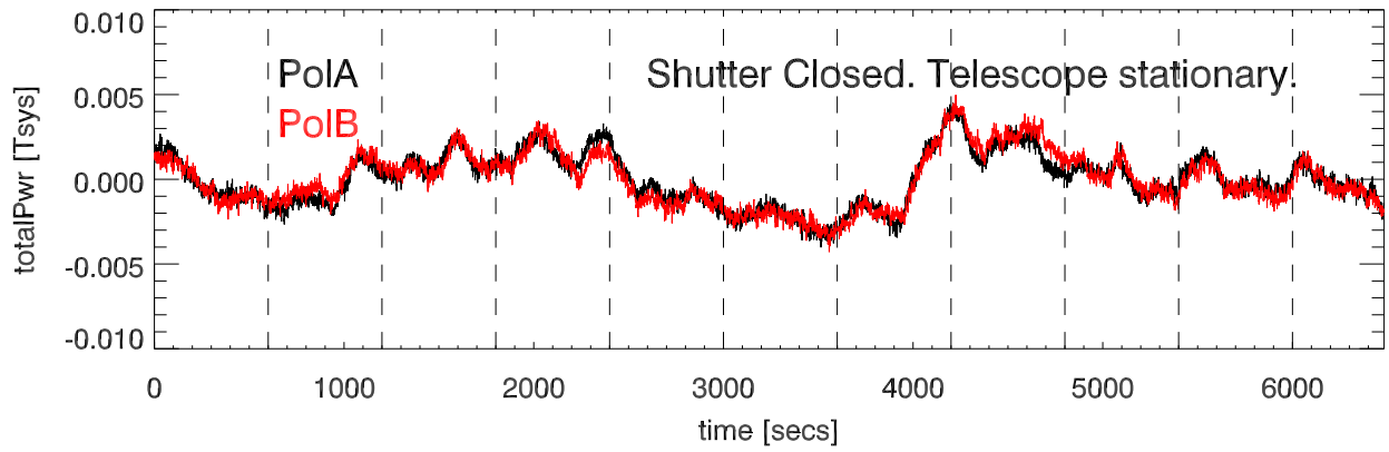
cband total power vs time. Remove2ndOrderFit. band0 Freq:4325 Mhz
