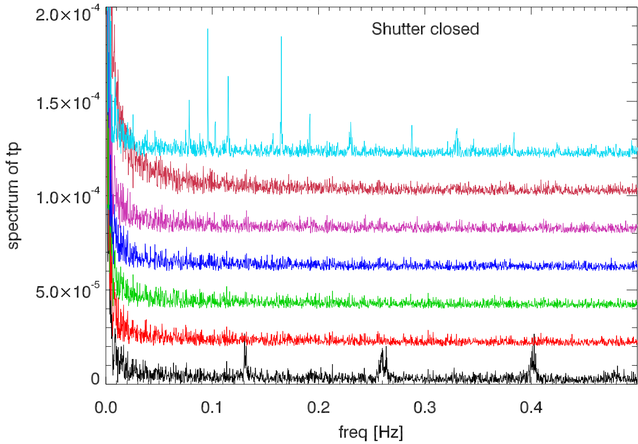
110209: cband spectrum of total power. PoIA
