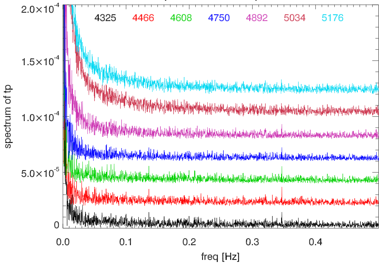
cband spectrum of total power. PoIB
