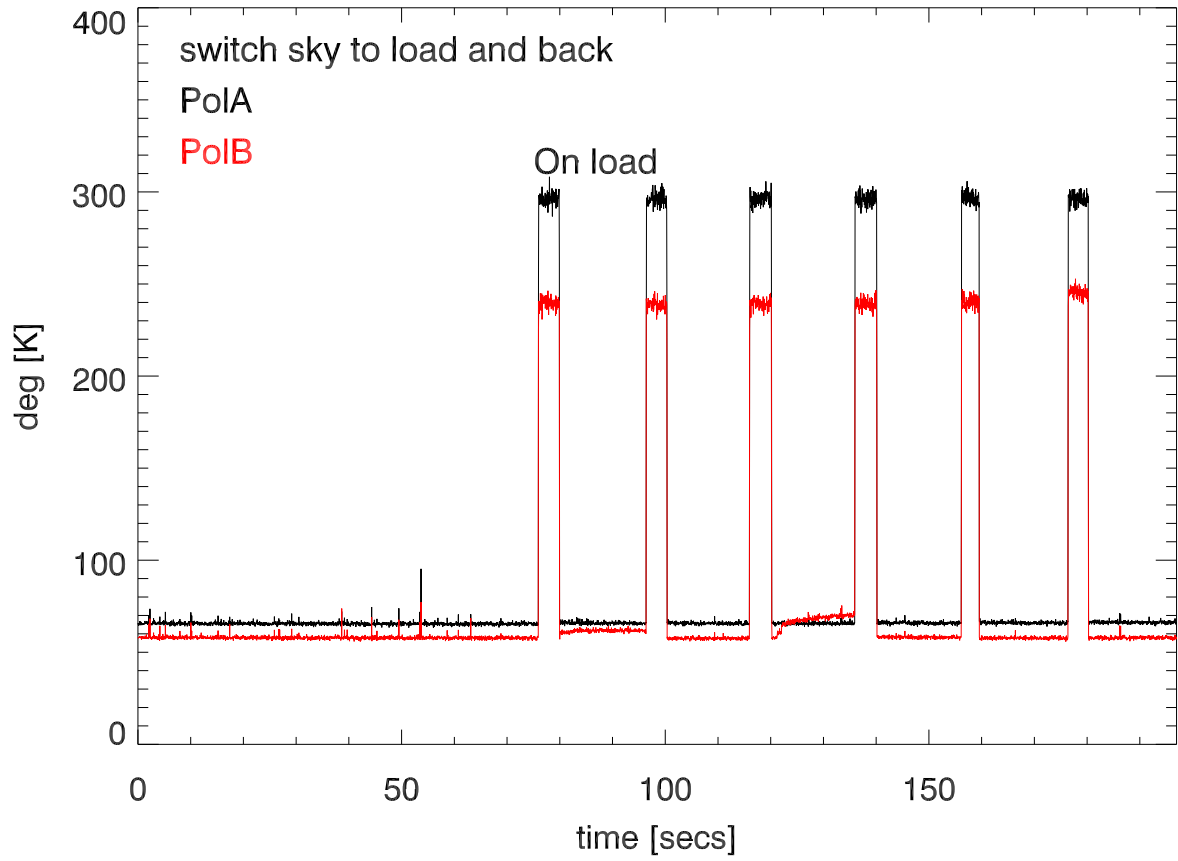
23apr19 gr430 tsys vs time
