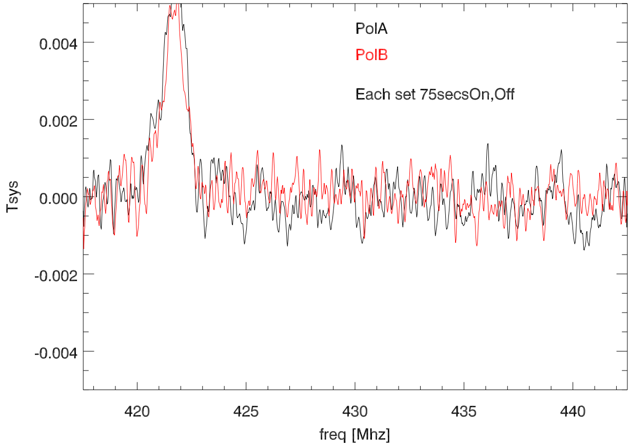
26mar12 430Dome. on/off-1.scan:5 set:1
