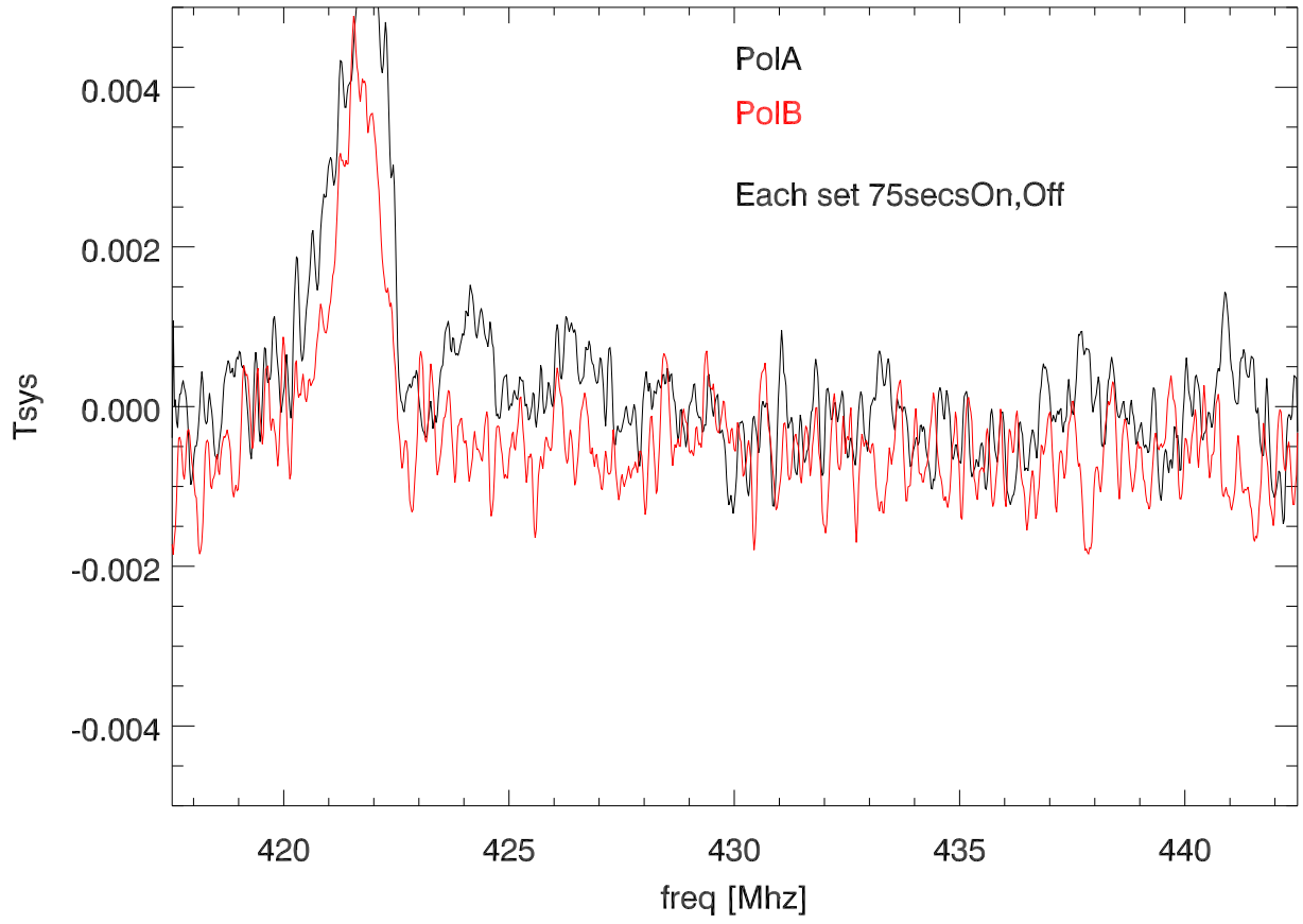
26mar12 430Dome. on/off-1.scan:3 set:1
