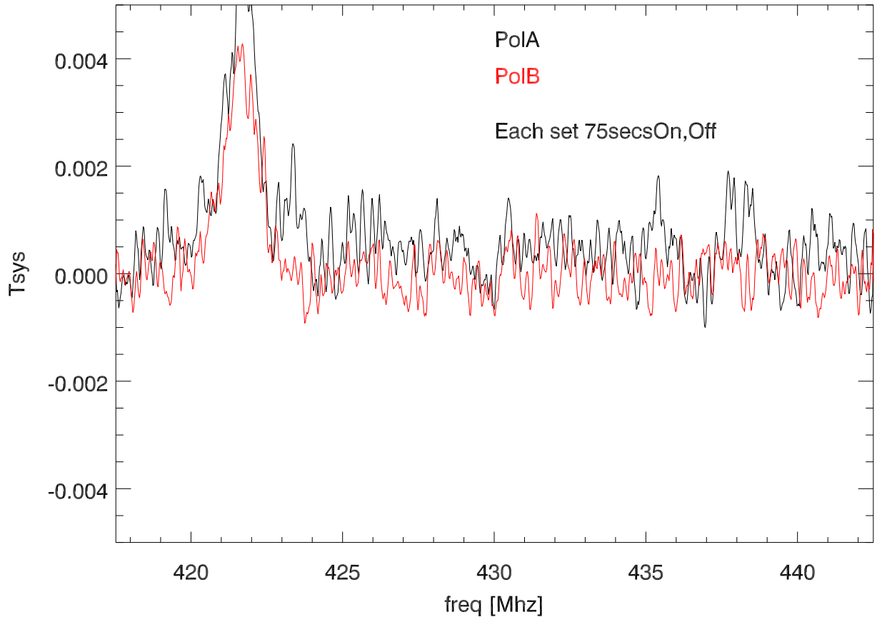
26mar12 430Dome. on/off-1.scan:6 set:1
