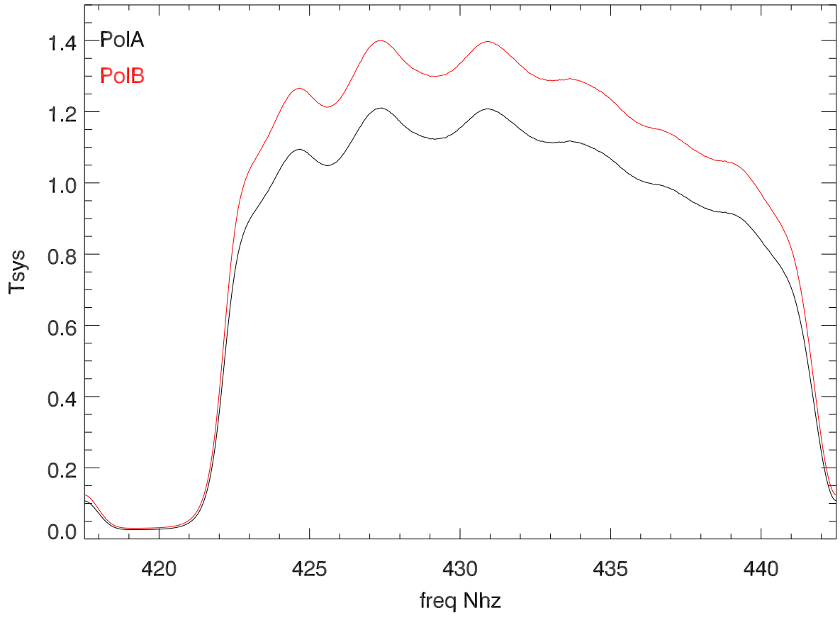
26mar12 430 dome. 75 second average spectra
