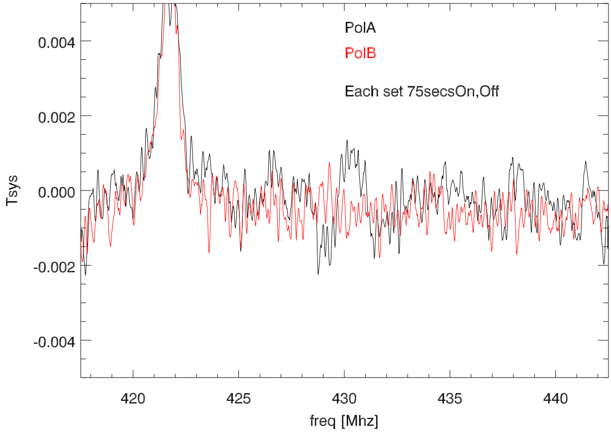
26mar12 430Dome. on/off-1.scan:2 set:1
