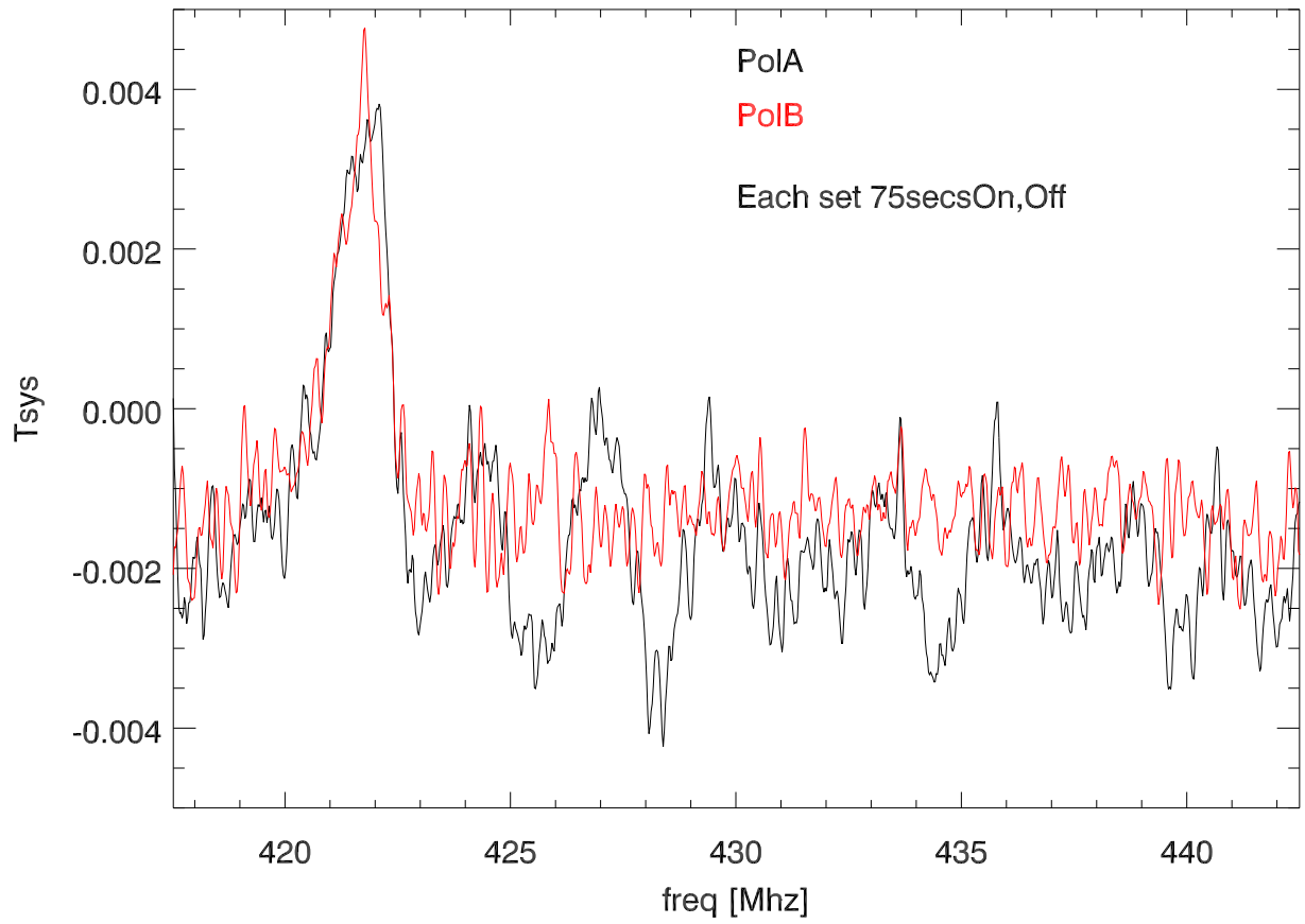
26mar12 430Dome. on/off-1.scan:1 set:1
