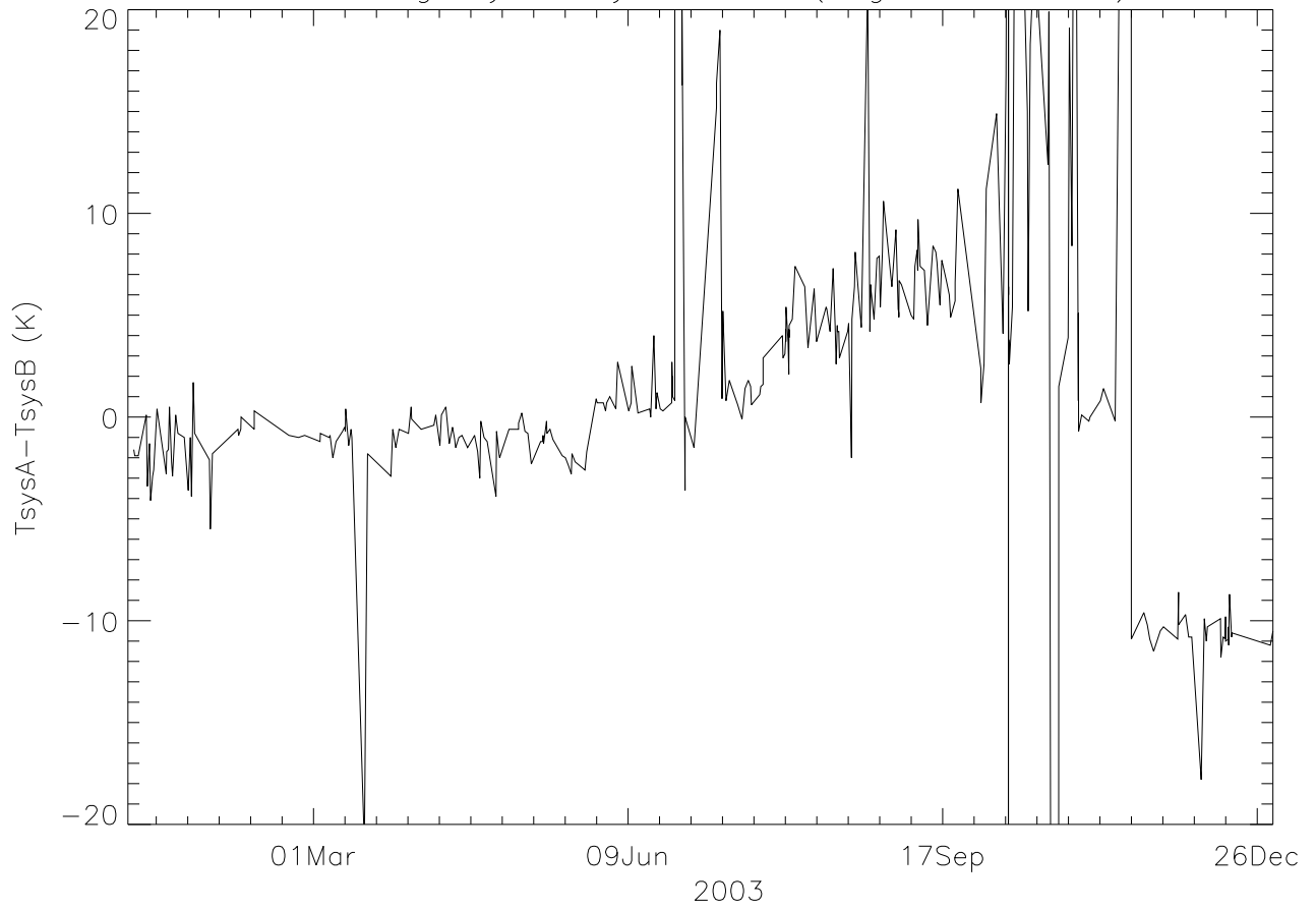
430 Greg T_{\text{sysA}} - T_{\text{sysB}} 2003. (avg over hi cal)
