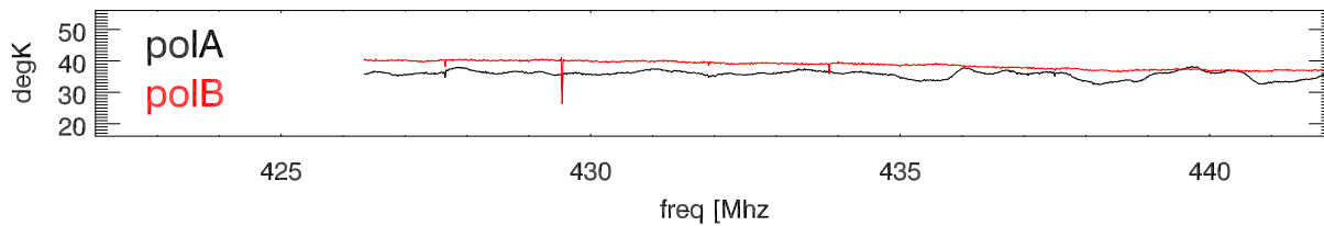
430Dome src Strength. B1559BP 2012-03-17
