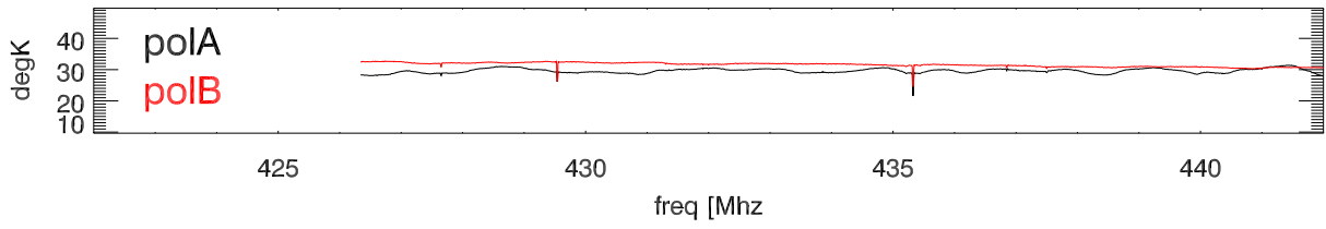
430Dome src Strength. B1559+140 2012-03-17
