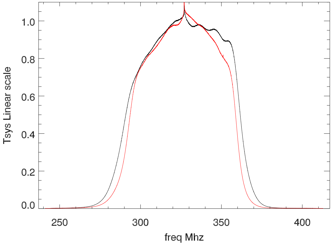
327 receiver showing cavity filter bandpass before dewar
