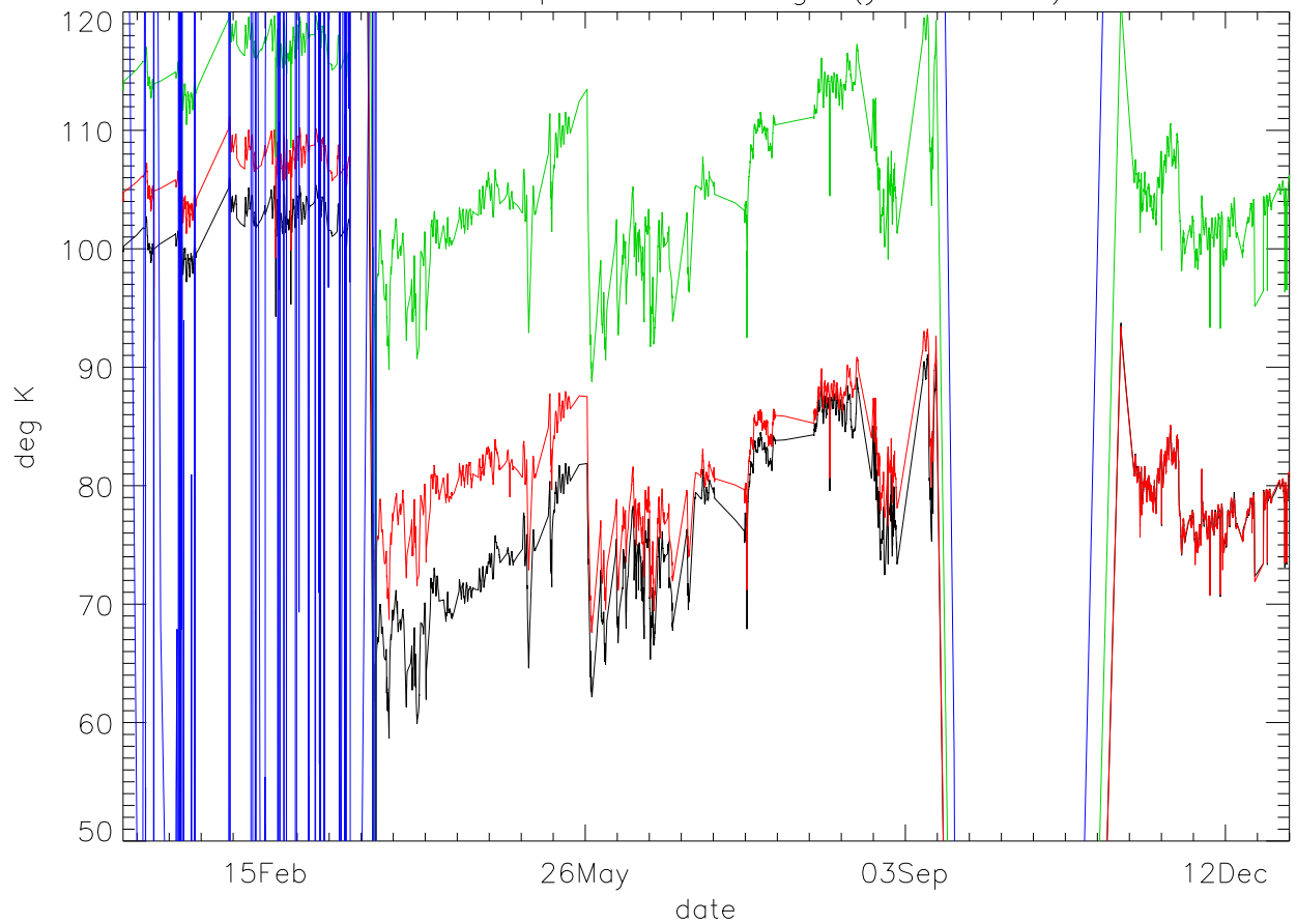
Dewar temps – 70K stage (year 2017)
