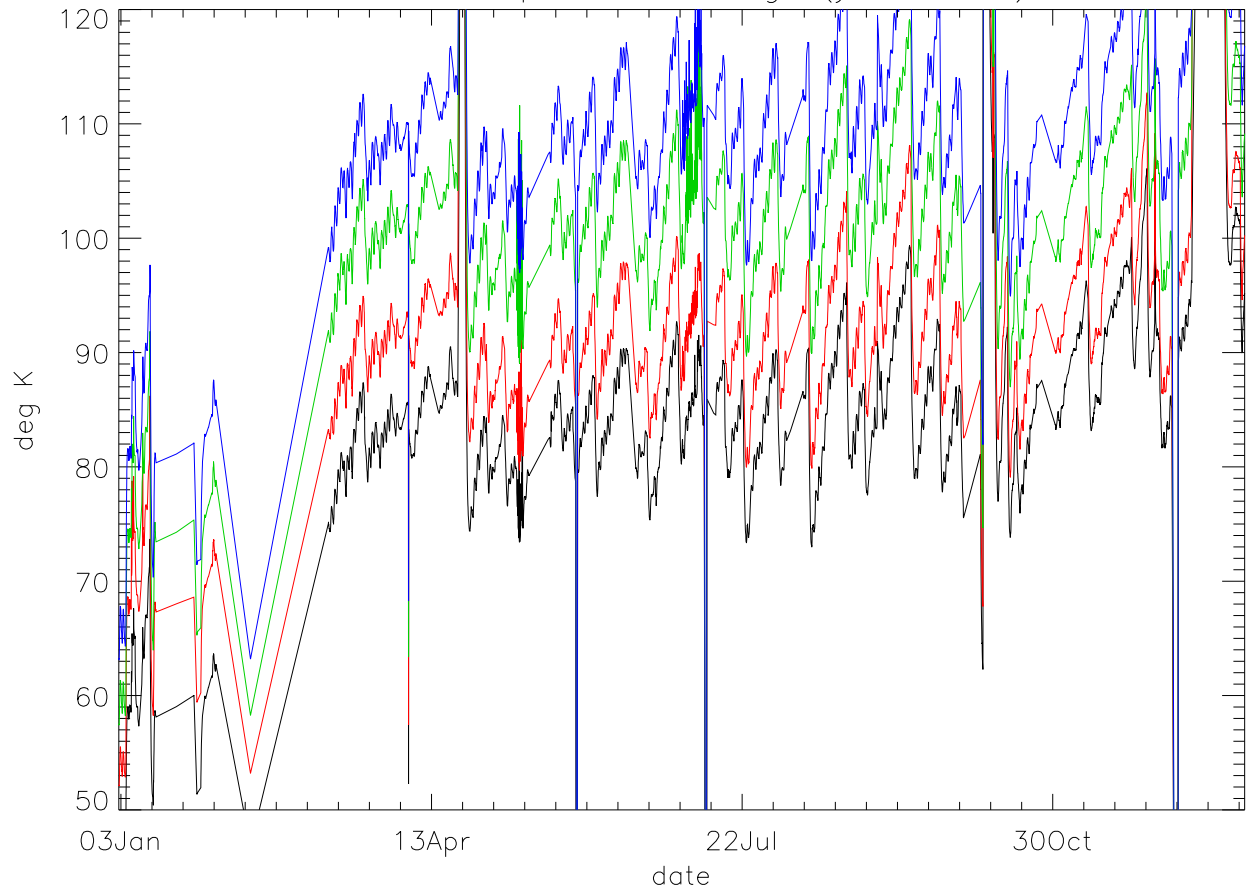
Dewar temps – 70K stage (year 2010)
