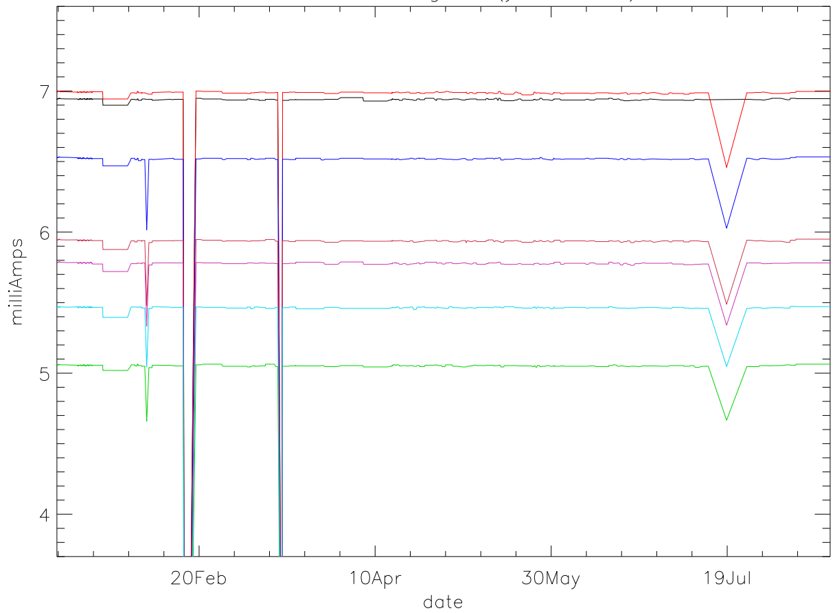
Id:Drain Current. stage 1 (year 2020) PoIB
