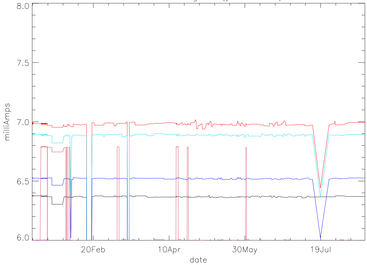
Id:Drain Current. stage 3 (year 2020) PoIB
