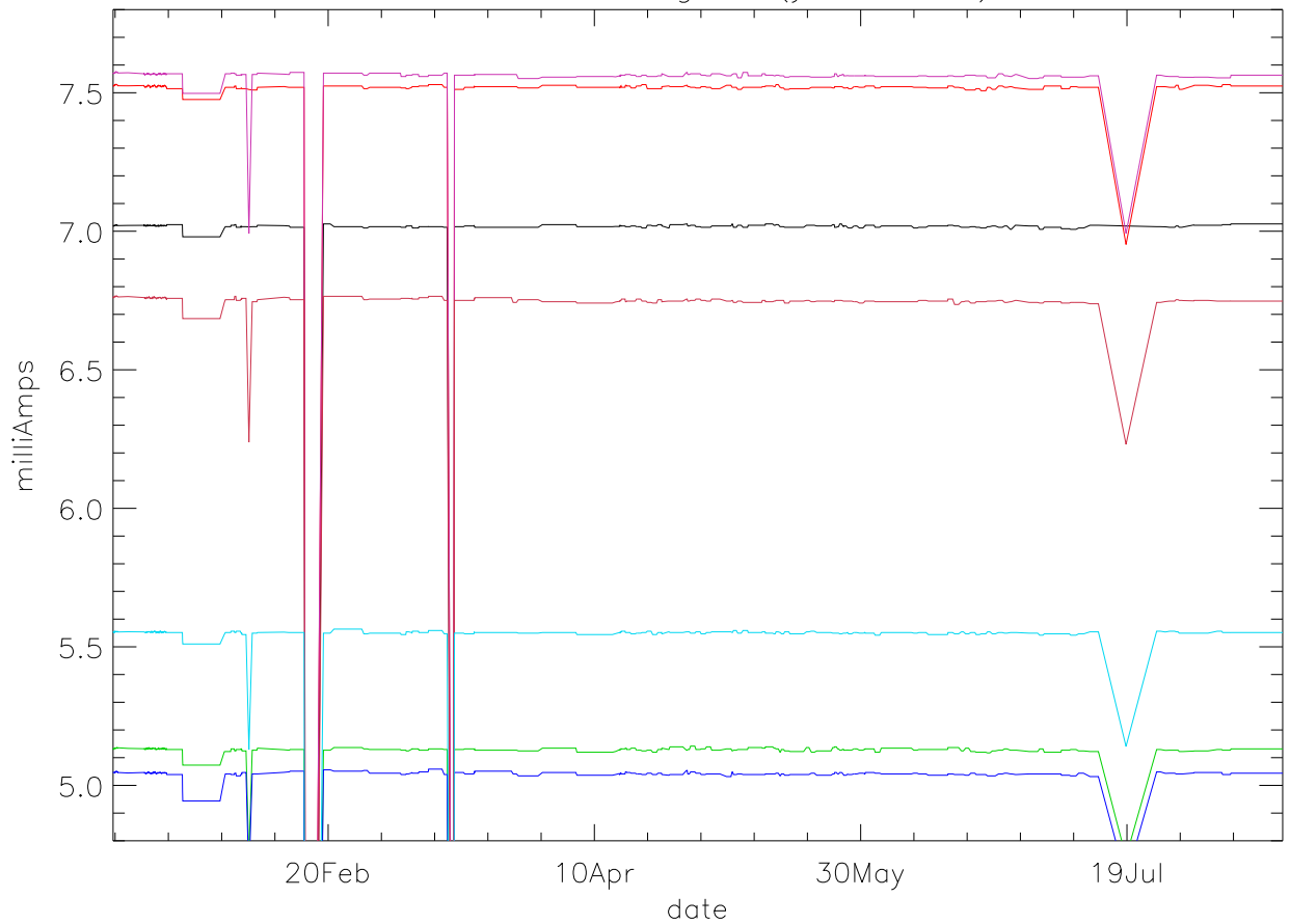
Id:Drain Current. stage 2 (year 2020) PoIB
