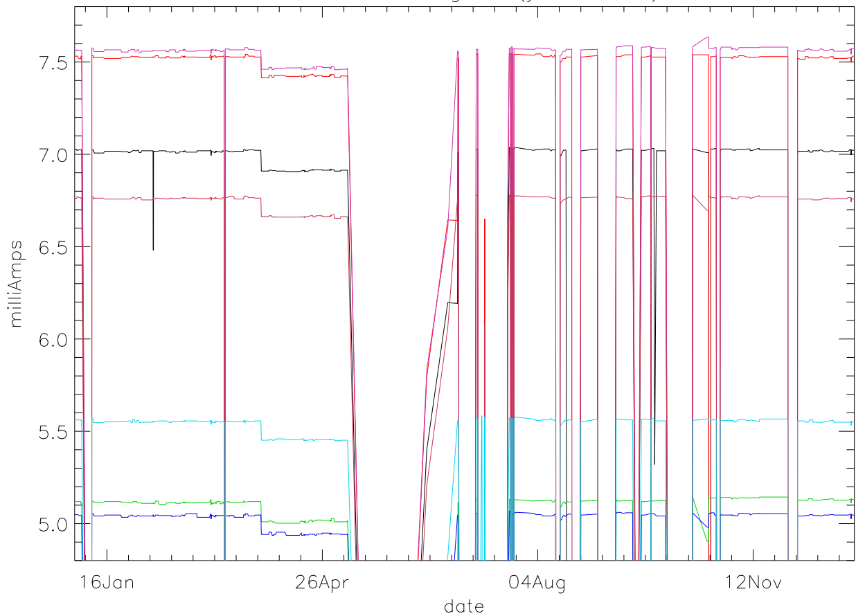
Id:Drain Current. stage 2 (year 2019) PoIB
