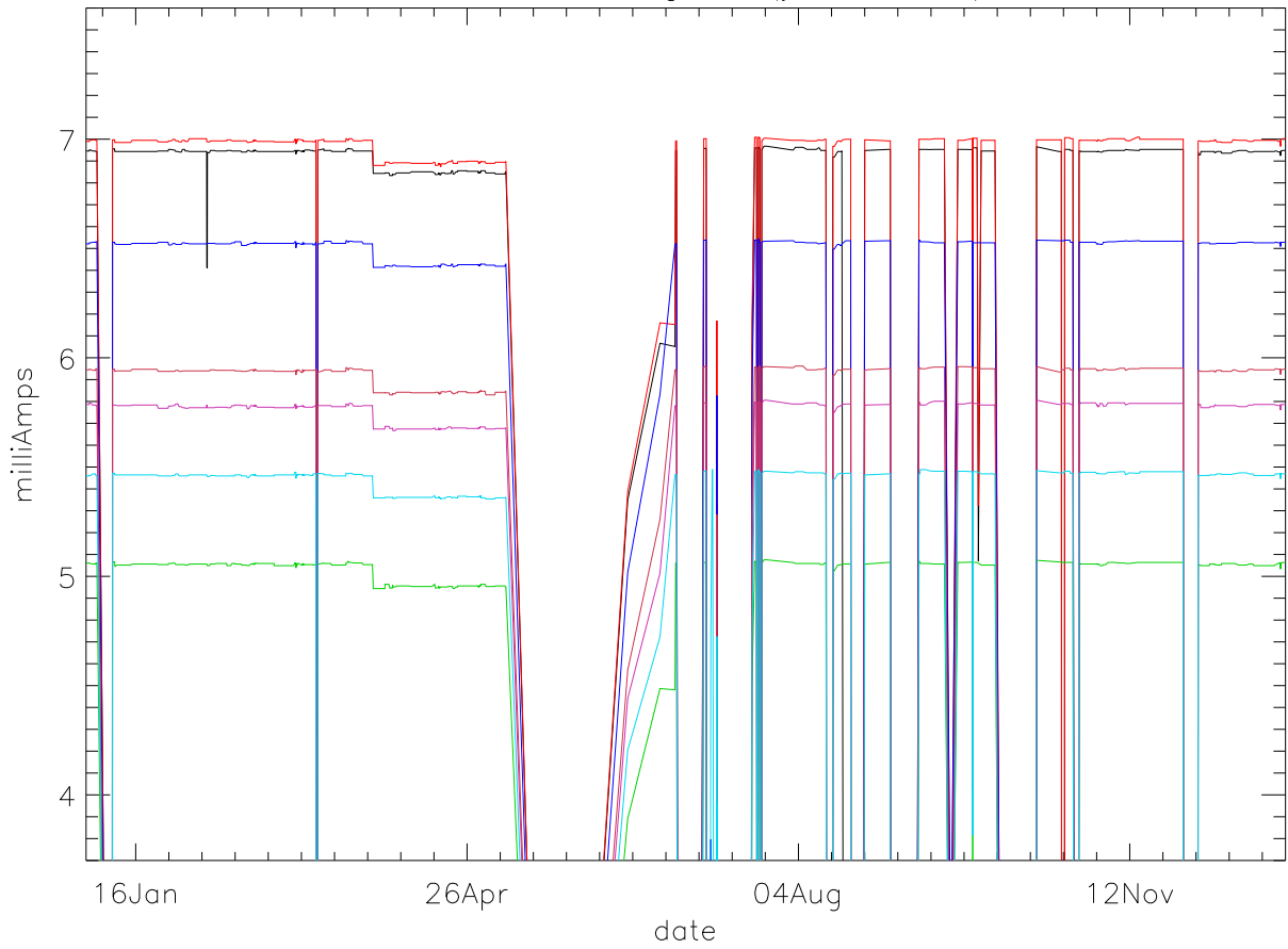
Id:Drain Current. stage 1 (year 2019) PoIB
