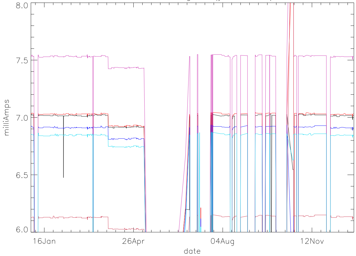
Id:Drain Current. stage 3 (year 2019) PoIB
