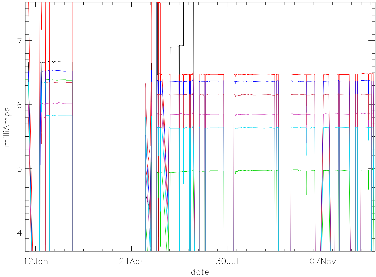
Id:Drain Current. stage 1 (year 2016) PoIB
