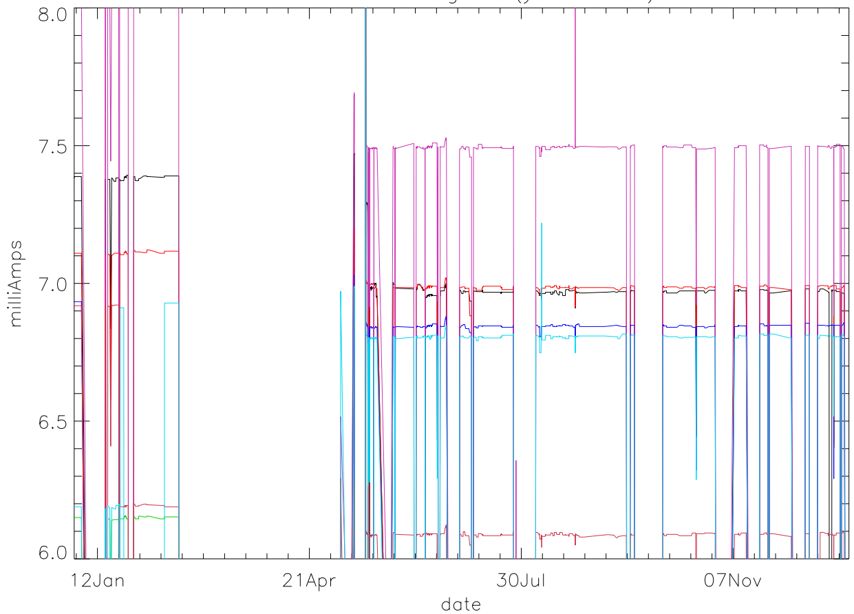
Id:Drain Current. stage 3 (year 2016) PoIB
