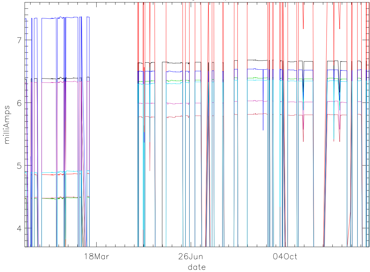
Id:Drain Current. stage 1 (year 2015) PoIB
