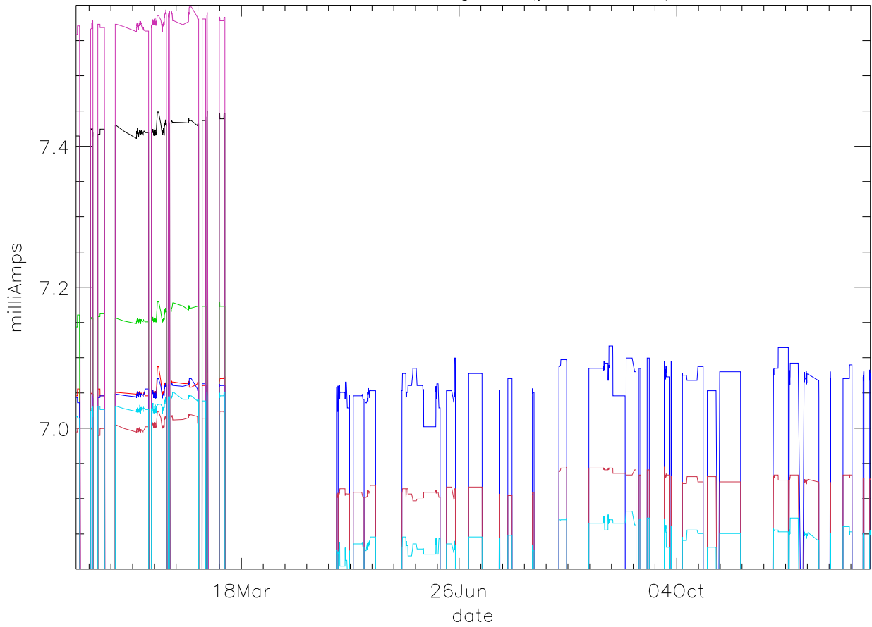
Id:Drain Current. stage 3 (year 2015) PoIB
