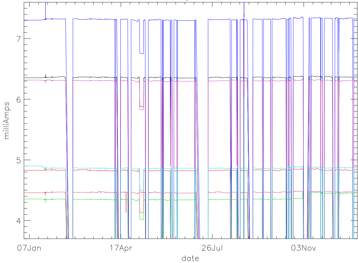
Id:Drain Current. stage 1 (year 2013) PoIB
