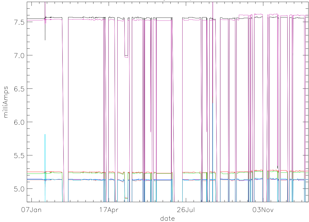
Id:Drain Current. stage 2 (year 2013) PoIB
