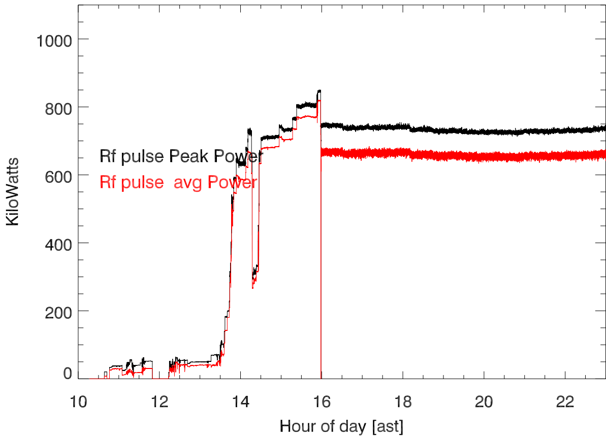
20190829 X110 430tx power (dome) vs hour of day
