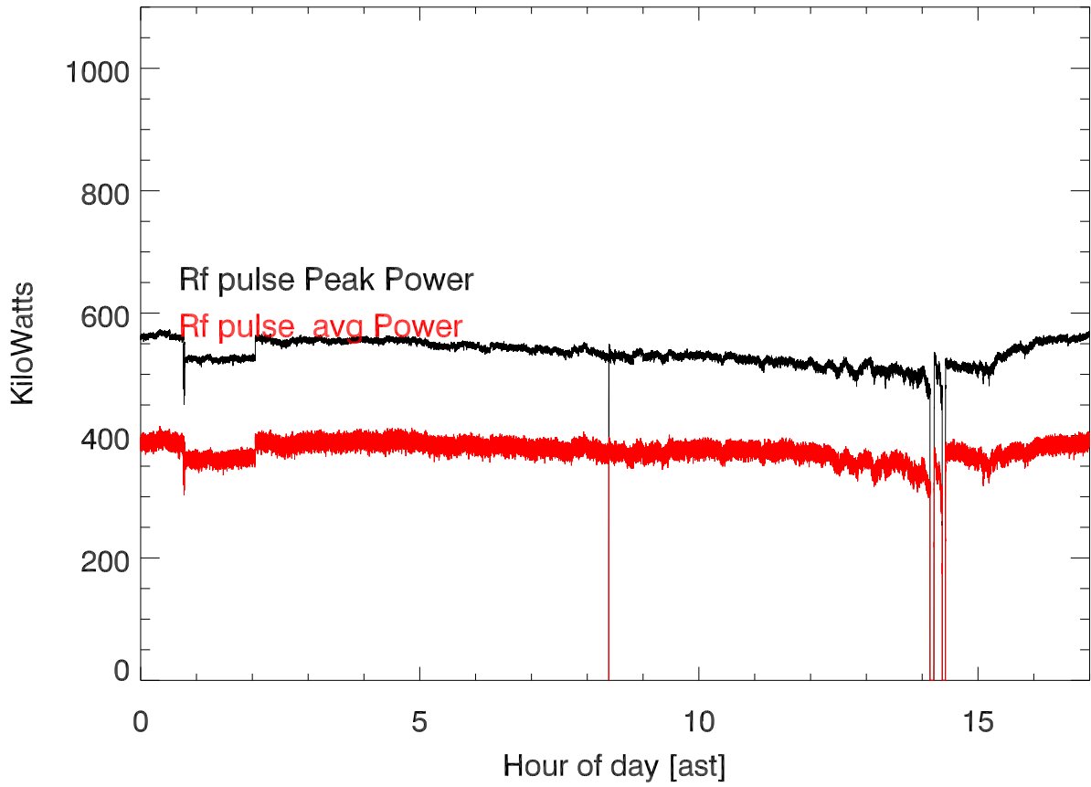
20190703 T3323 430tx power (dome) vs hour of day
