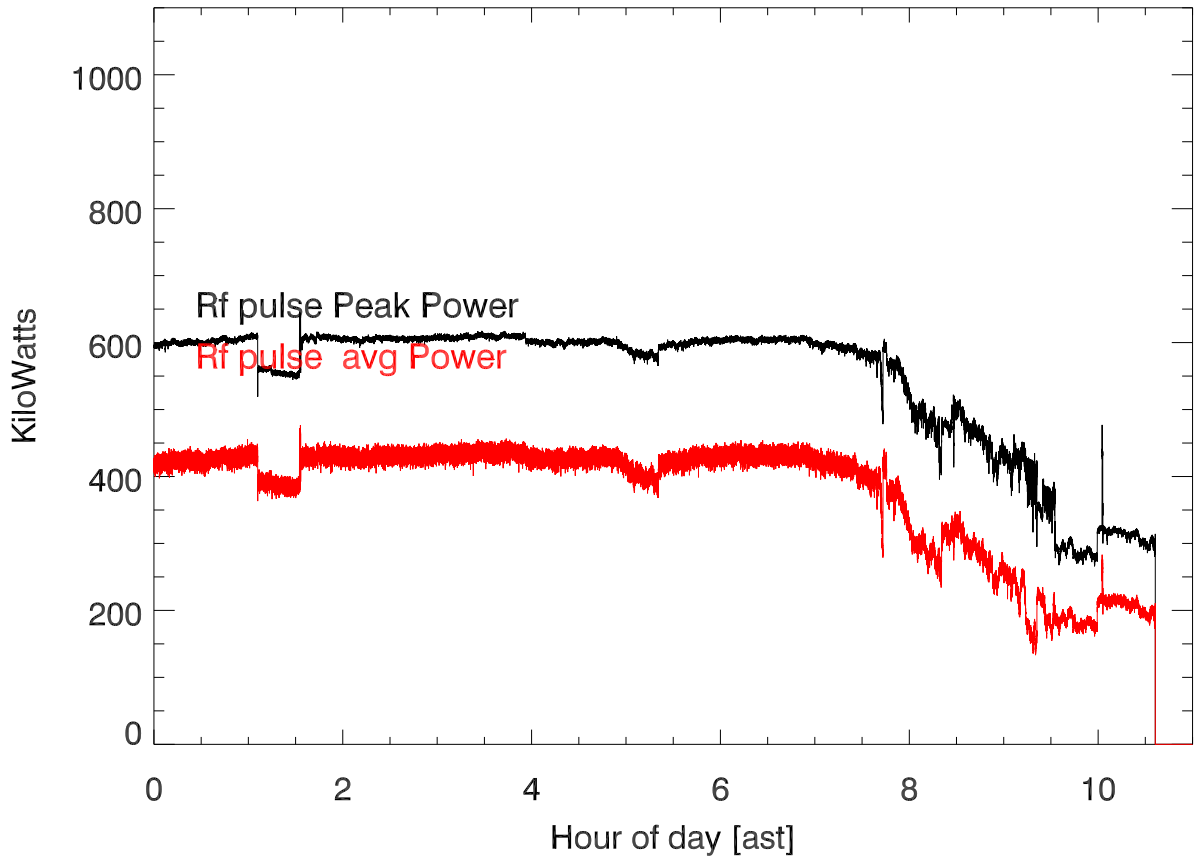
20190704 T1193 430tx power (dome) vs hour of day
