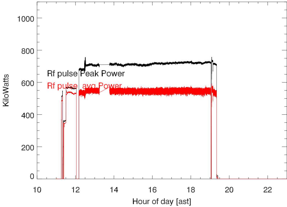
20190629 T3323 430tx power (dome) vs hour of day
