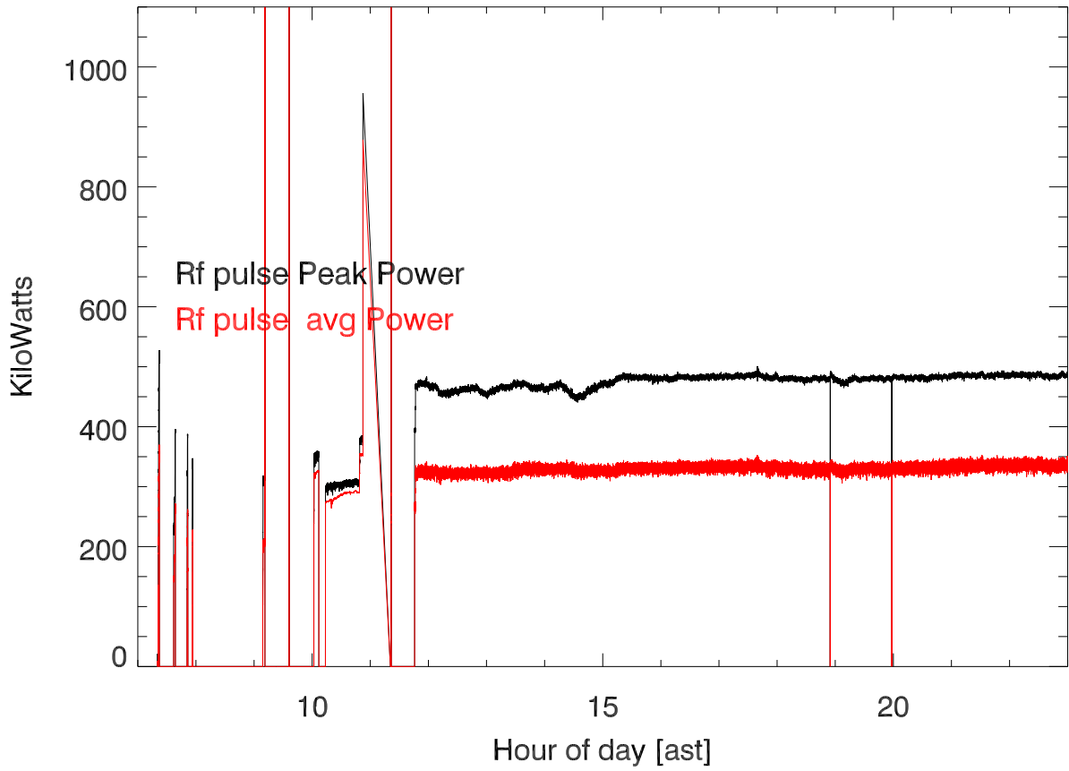
20190705 T3323 430tx power (dome) vs hour of day
