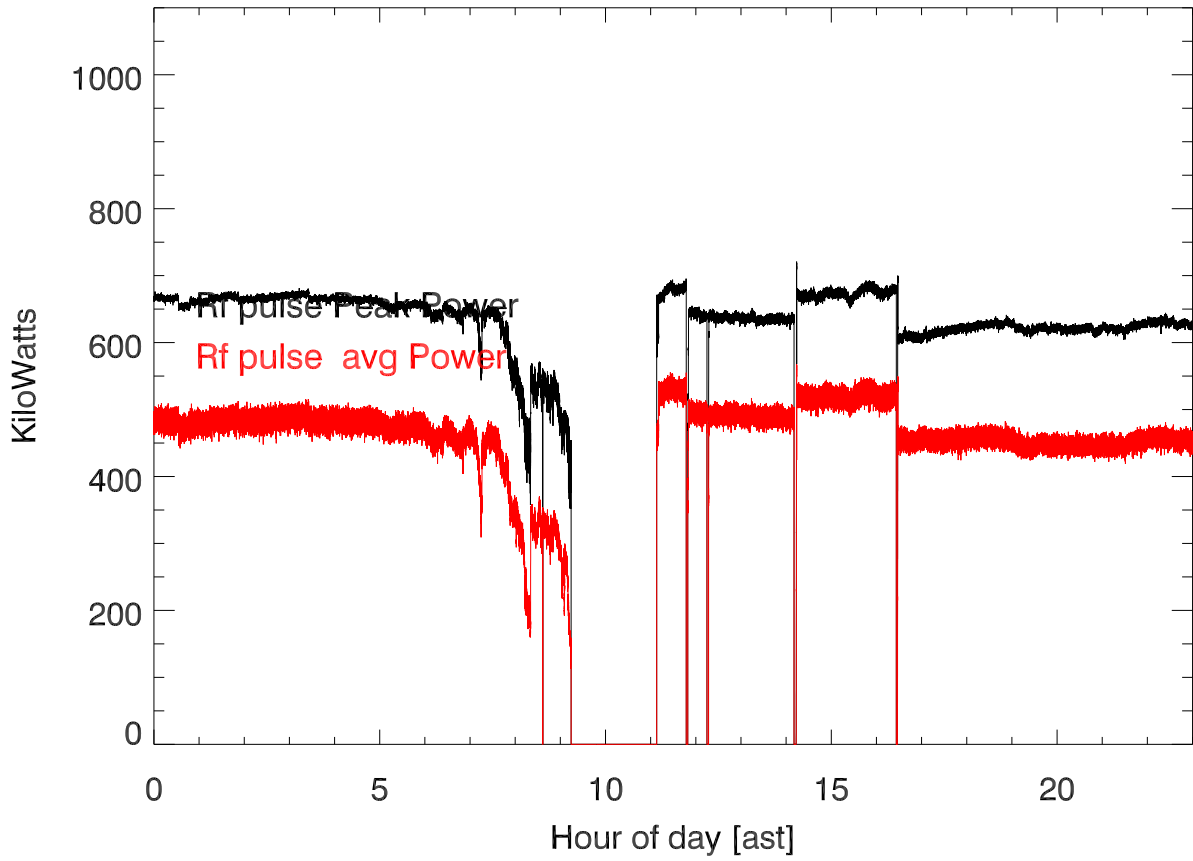
20190701 T3323 430tx power (dome) vs hour of day
