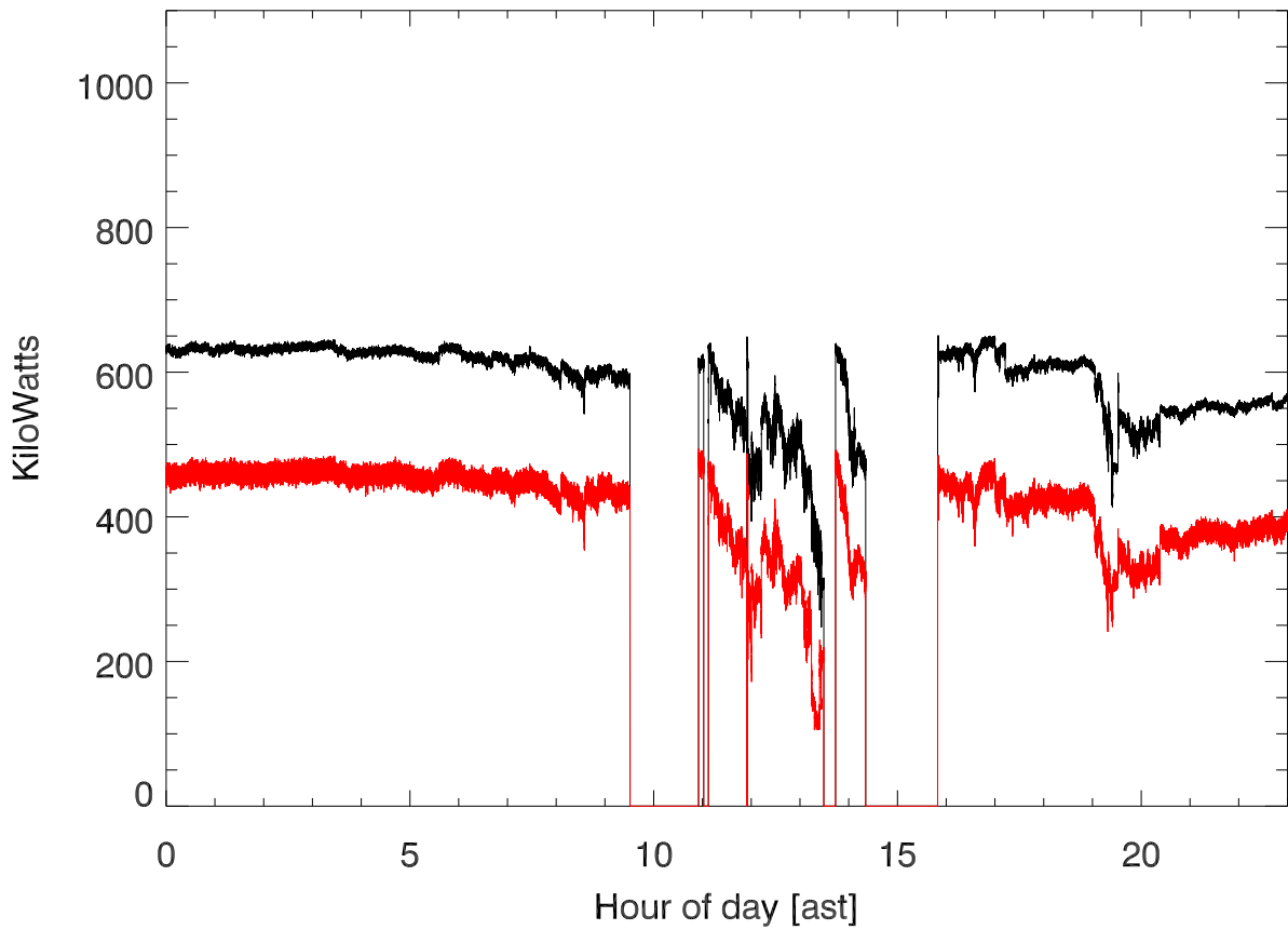
20190702 T3323 430tx power (dome) vs hour of day
