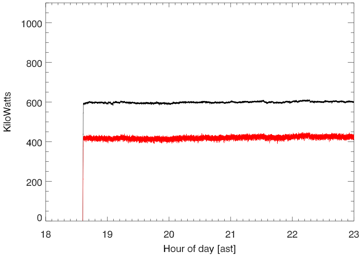
20190703 T1193 430tx power (dome) vs hour of day
