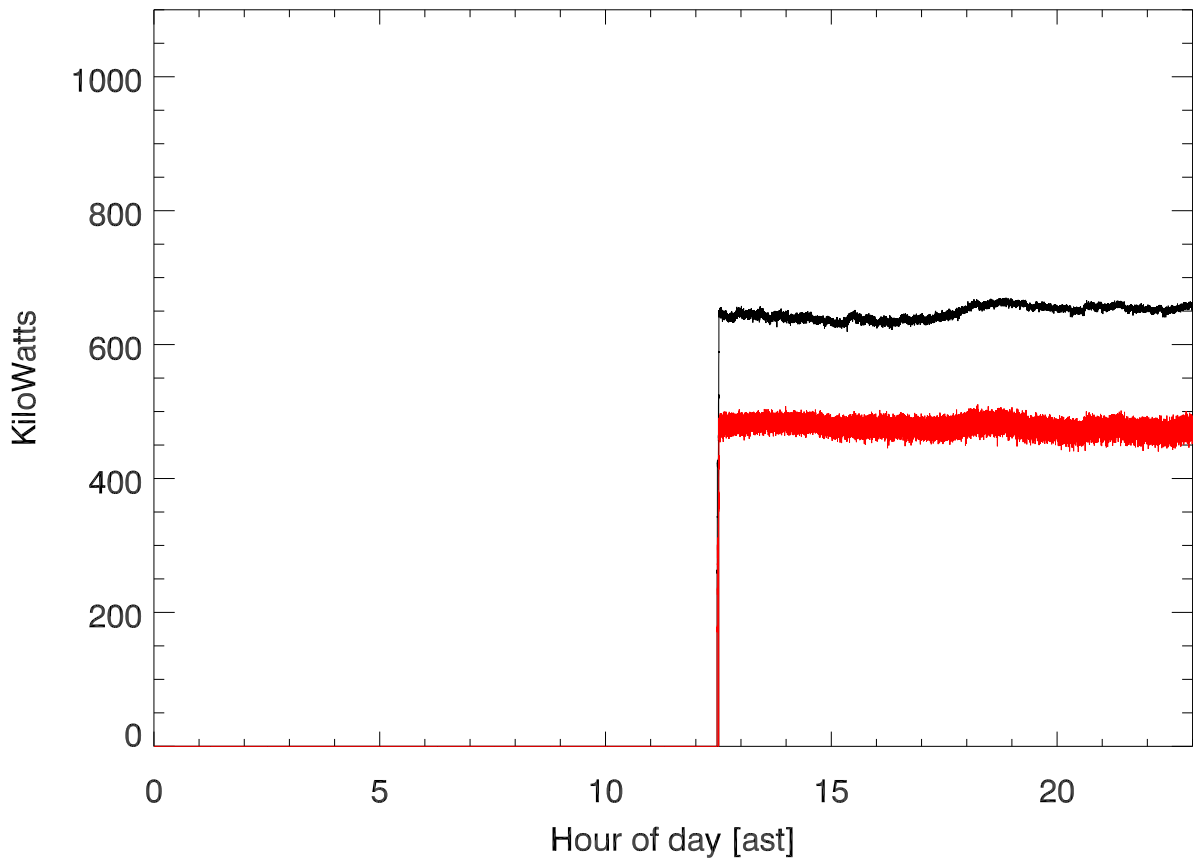
20190630 T3323 430tx power (dome) vs hour of day
