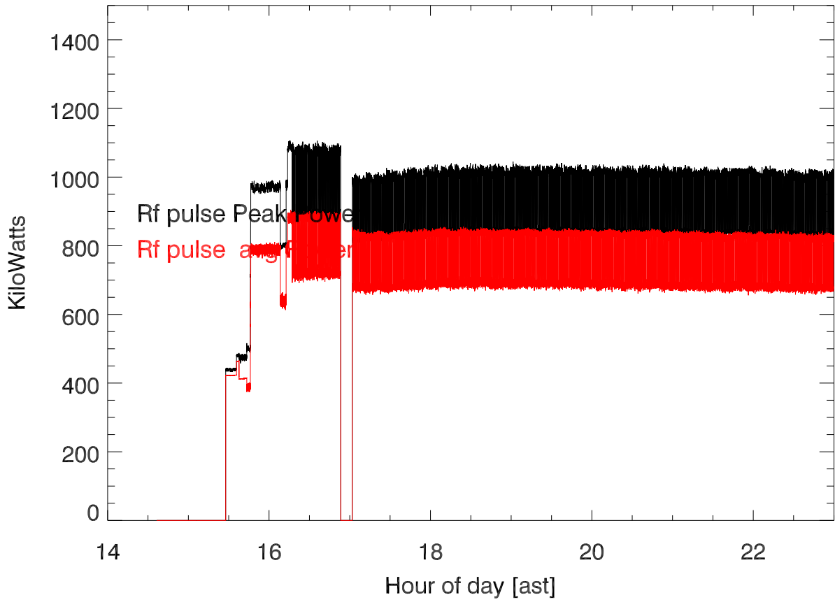
20190104 t3150 430tx power (dome) vs hour of day
