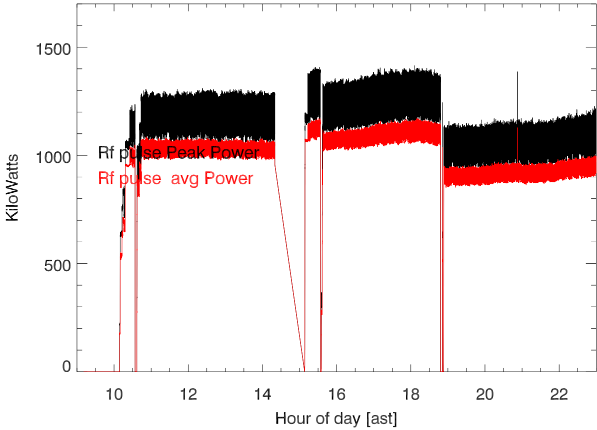
20180129 T1193 430tx power (dome) vs hour of day
