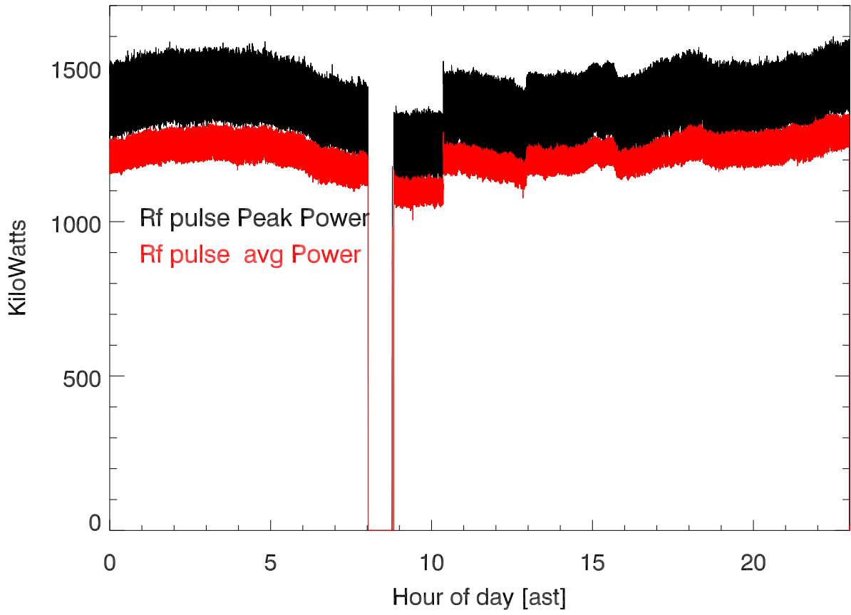
20180131 T1193 430tx power (dome) vs hour of day
