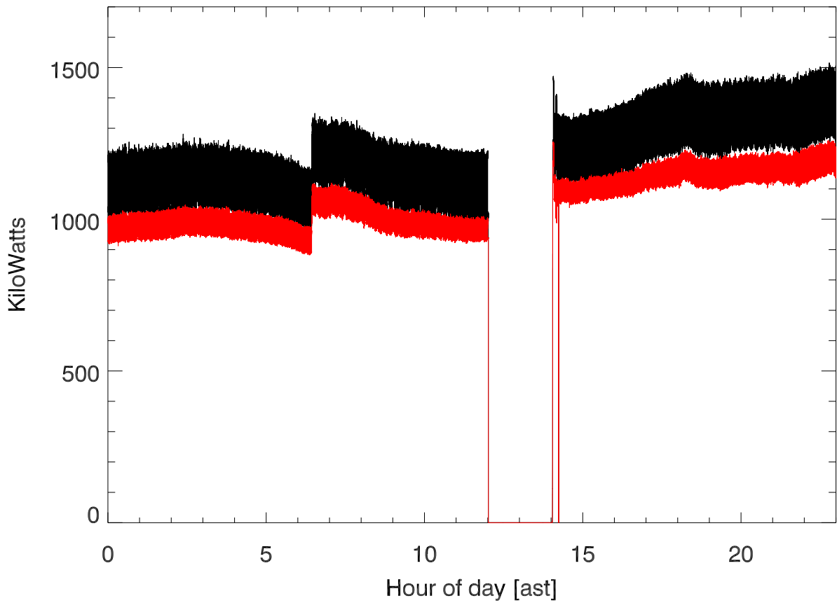
20180130 T1193 430tx power (dome) vs hour of day
