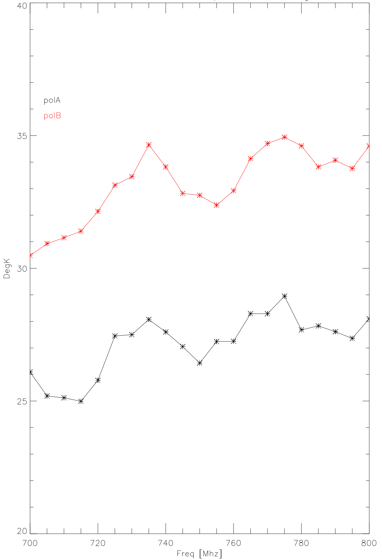
800Rcvr calValues vs Freq measured 13aug09
