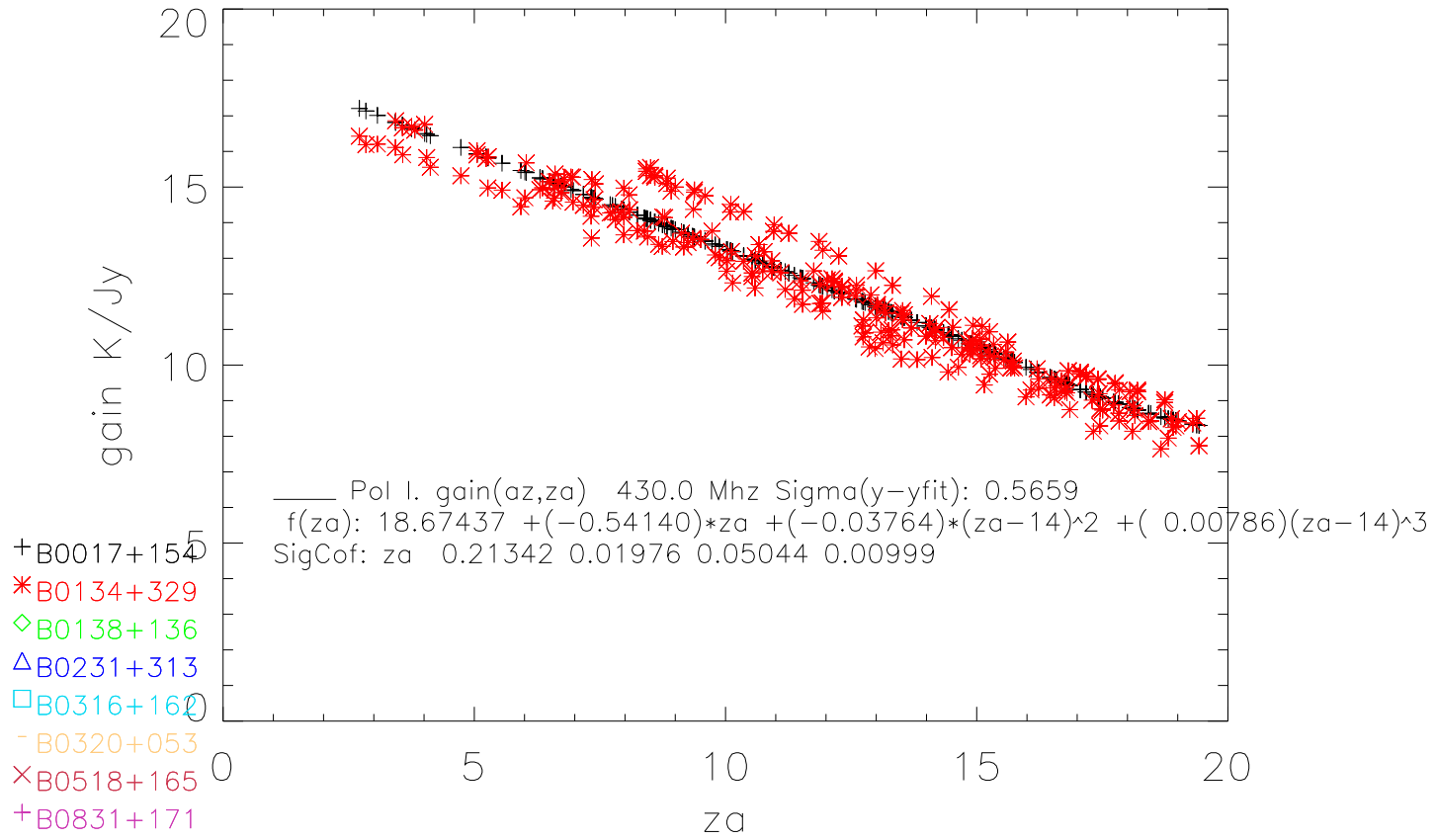
ch gain vs za and fit mar05
