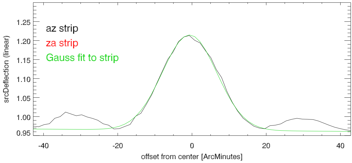
18mar19: Az,Za cross patterns on B0240-002 Az strip Pattern: 2
