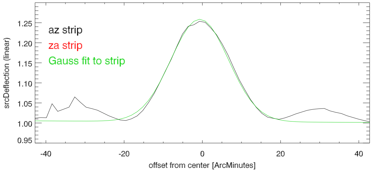
18mar19: Az,Za cross patterns on B0240-002 Az strip Pattern: 4
