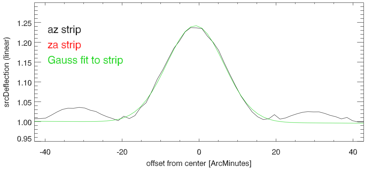
18mar19: Az,Za cross patterns on B0240-002 Az strip Pattern: 6
