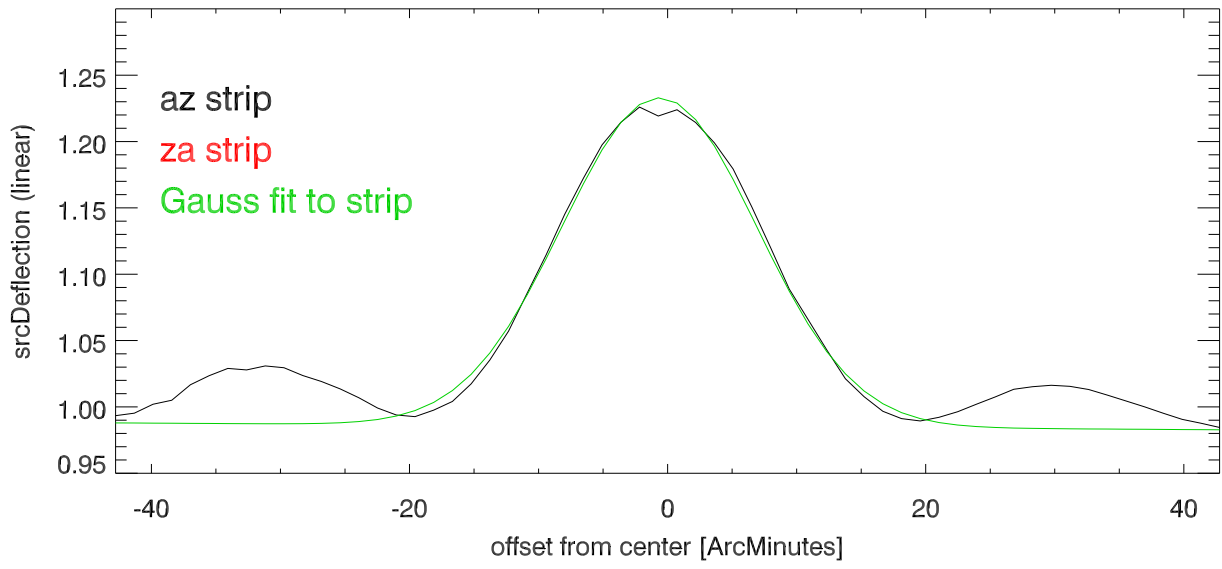
18mar19: Az,Za cross patterns on B0240-002 Az strip Pattern: 3
