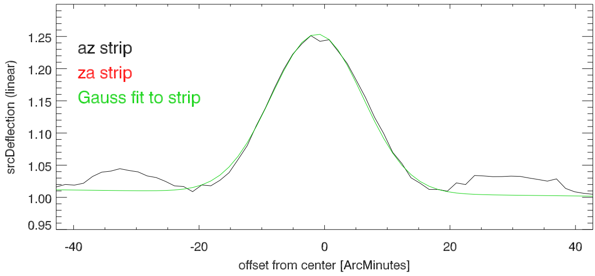
18mar19: Az,Za cross patterns on B0240-002 Az strip Pattern: 7
