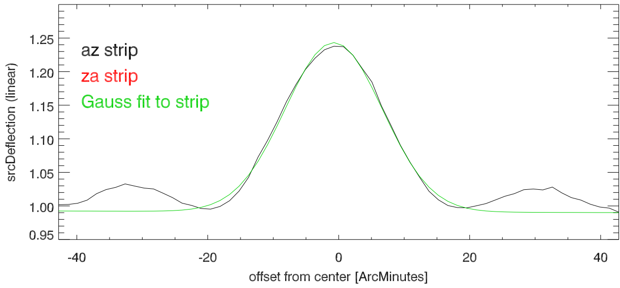
18mar19: Az,Za cross patterns on B0240-002 Az strip Pattern: 5
