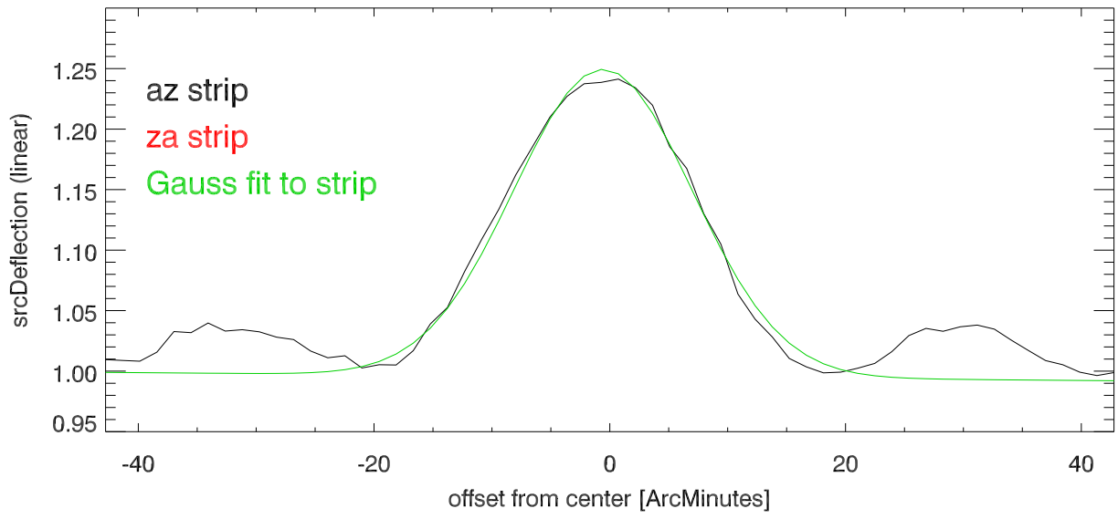
18mar19: Az,Za cross patterns on B0240-002 Az strip Pattern: 1
